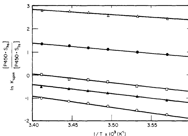
FIGURE 2: Equilibrium constant as a function of temperature for camphor ( \Delta ), camphoroquinone ( \bullet ), fenchone ( \square ), norcamphor ( \blacktriangle ), and tetramethylcyclohexanone ( \circ ) bound forms of cytochrome P-450 cam . The temperature-induced optical changes were analyzed by using the methods outlined under Materials and Methods.
